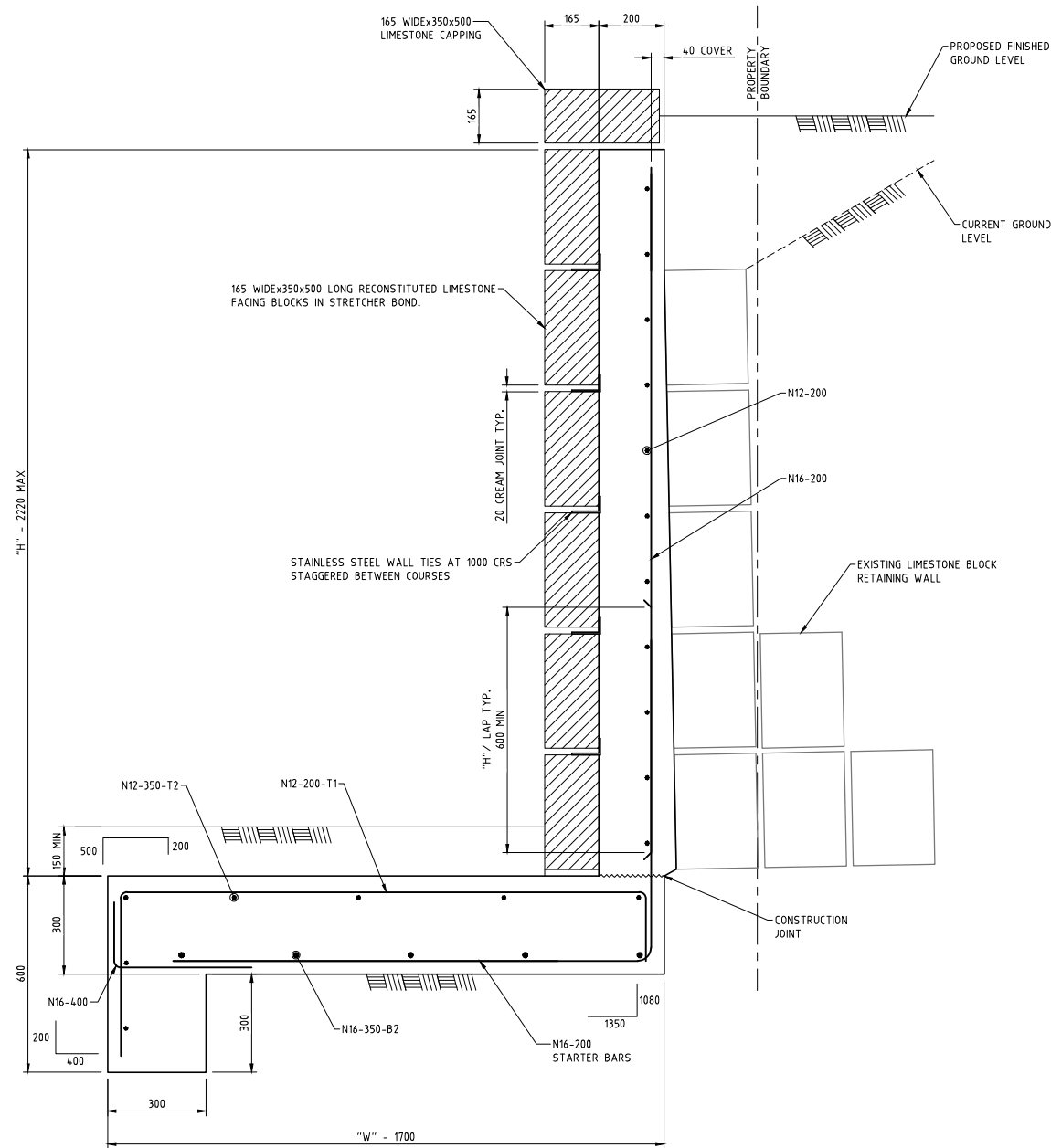
SECTION A OPTION 1 1:10
